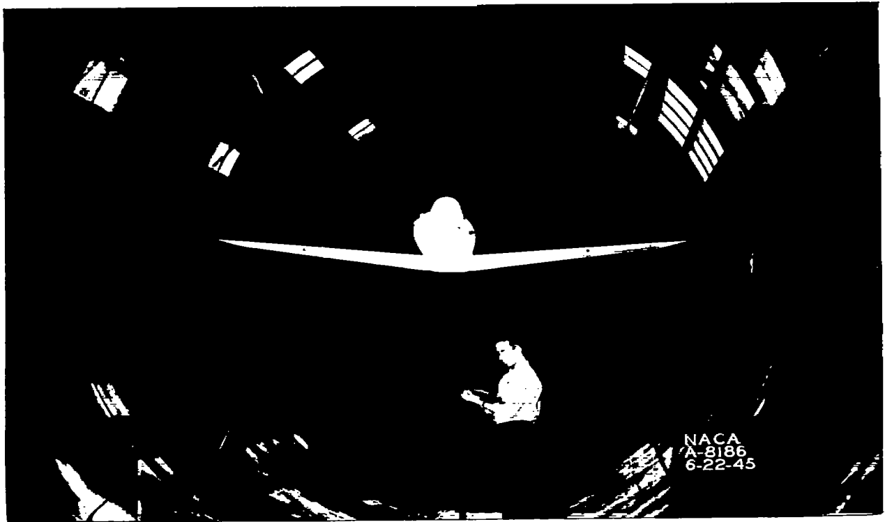
(a) Front view of the P-39N-1 model mounted in the tunnel.
