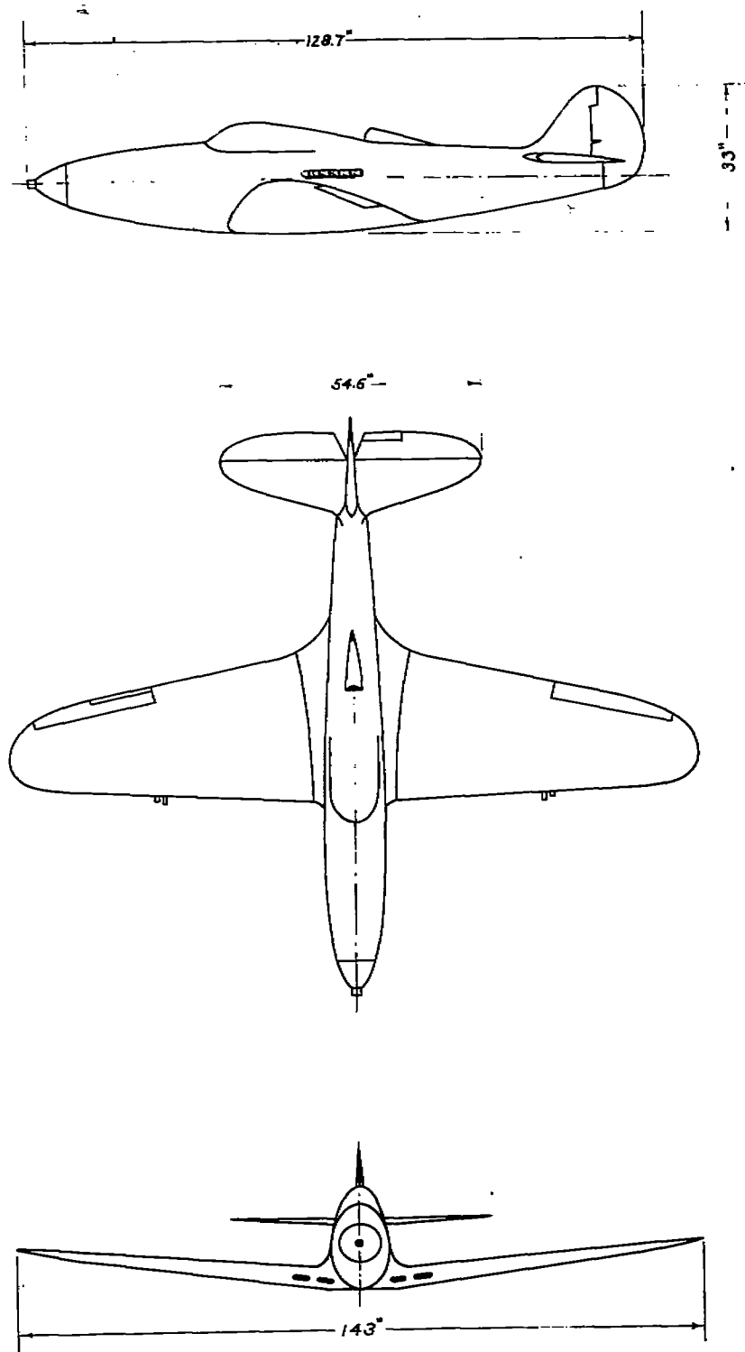
FIGURE 1.- THREE-VIEW DRAWING OF THE .35 SCALE MODEL OF THE P-39N-1 AIRPLANE.
