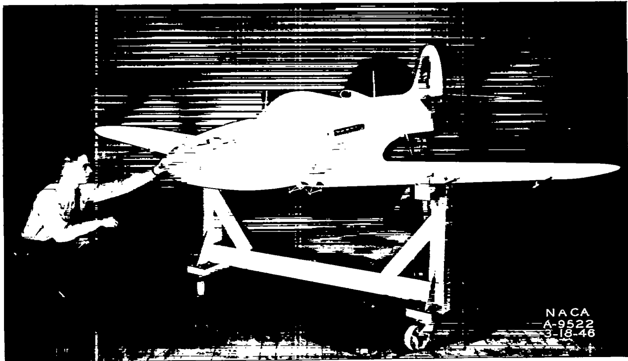
(b) Three-quarter front view of the P-39N-1 model showing accessories in place.
