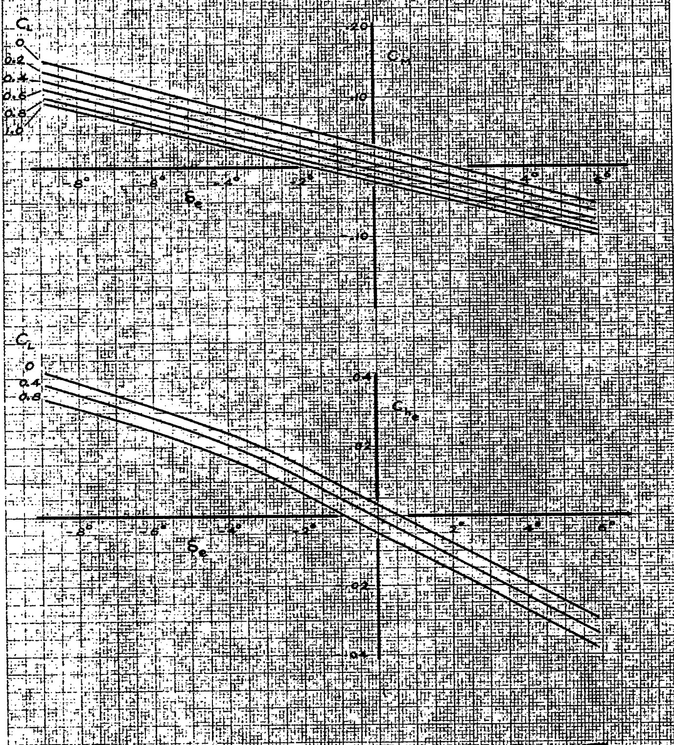
FIGURE 11 - VARIATION OF PITCHING-MOMENT AND ELEVATOR-HINGE-MOMENT COEFFICIENTS WITH ELEVATOR ANGLE FOR CONSTANT LIFT COEFFICIENTS, THEORETICAL ELEVATORS, \alpha = 2\frac{1}{4}^\circ ; \delta_e = 0^\circ ; P-39N-1 MODEL
