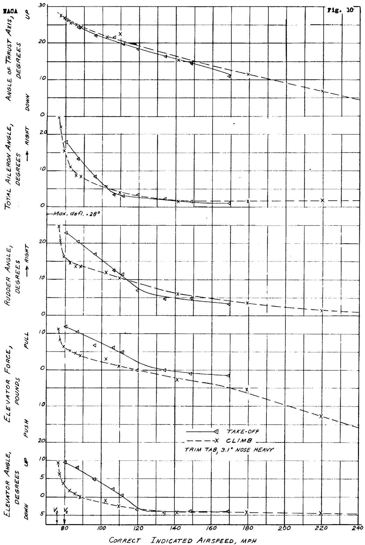
Figure 10. - Static longitudinal-stability characteristics of the Supermarine Spitfire airplane MMG in the climbing and take-off conditions.
